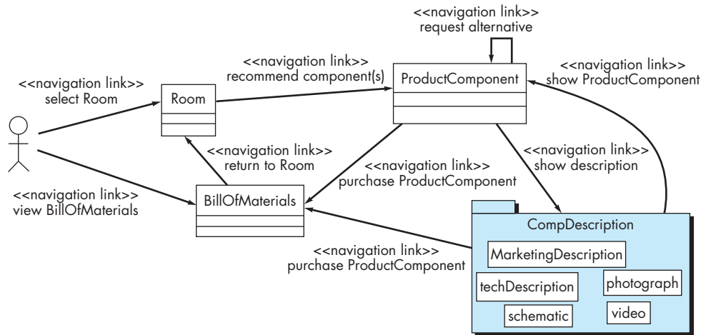
FIGURE 17.9 Creating an NSU
