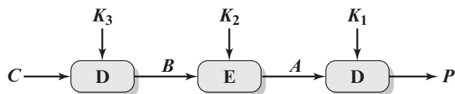
(b) Decryption
