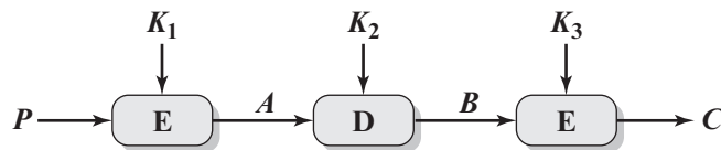
(a) Encryption
