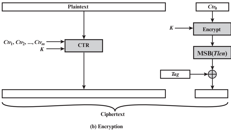
Figure 3.8 Counter with Cipher Block Chaining-Message Authentication Code
