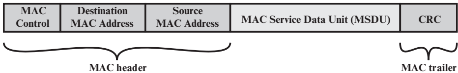
Figure 7.4 General IEEE 802 MPDU Format
