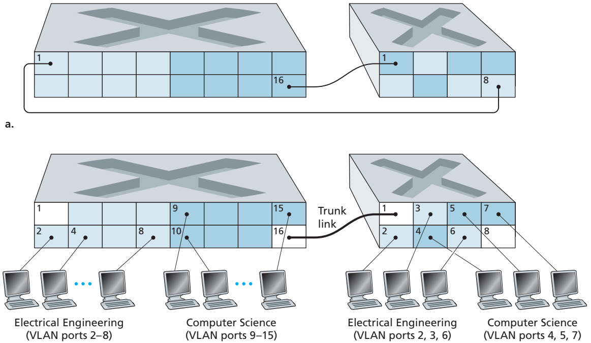
Figure 5.26 ♦ Connecting two VLAN switches with two VLANs: (a) two cables (b) trunked
