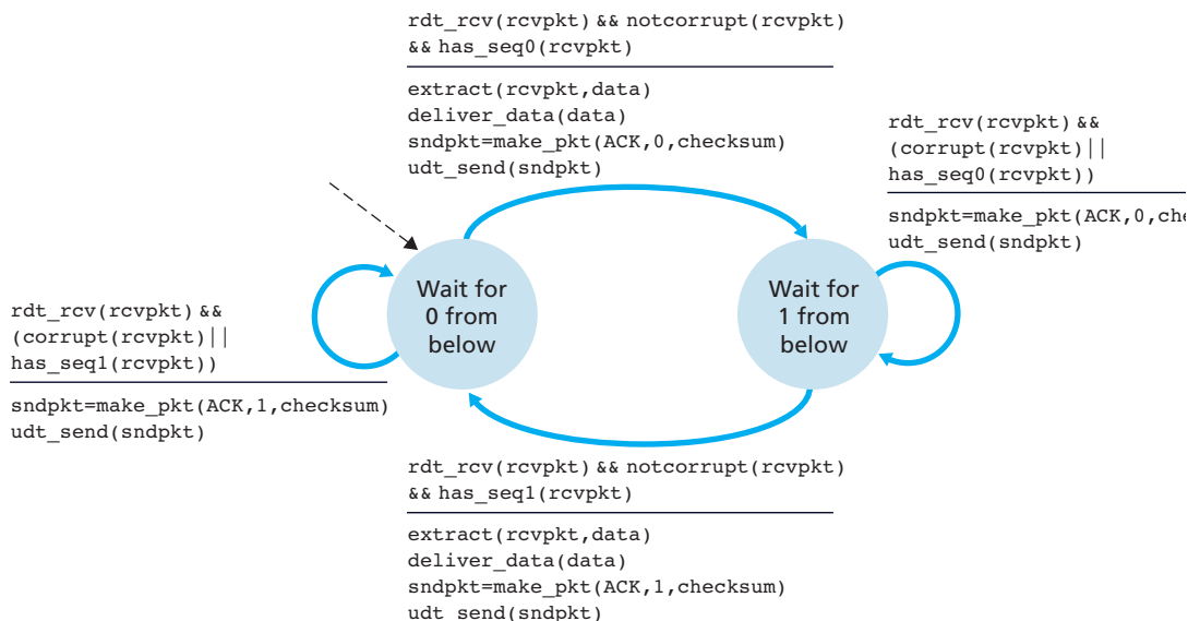
Figure 3.14 ♦ rdt2.2 receiver
