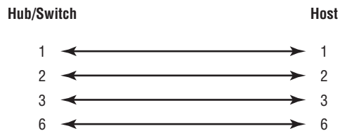
FIGURE 3.21 Straight-through Ethernet cable
