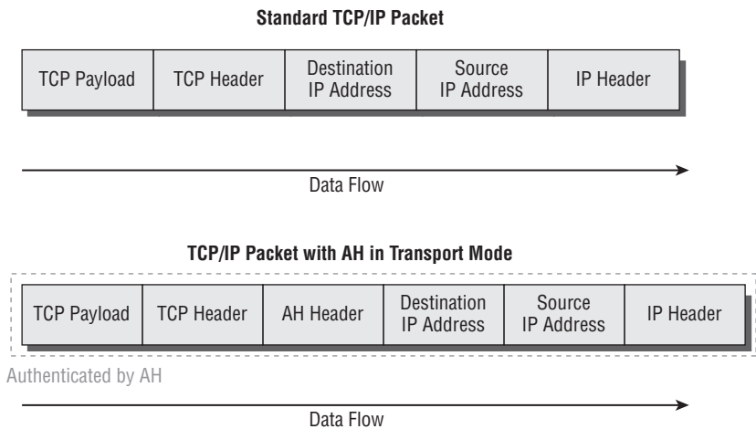
FIGURE 13.5 TCP/IP packet in IPSec transport mode with AH
