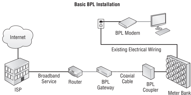
FIGURE 3.15 Basic BPL installation
