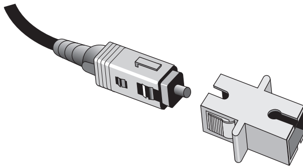
FIGURE 3.7 A sample SC connector
