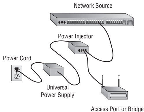
FIGURE 11.19 An external power injector used for PoE
