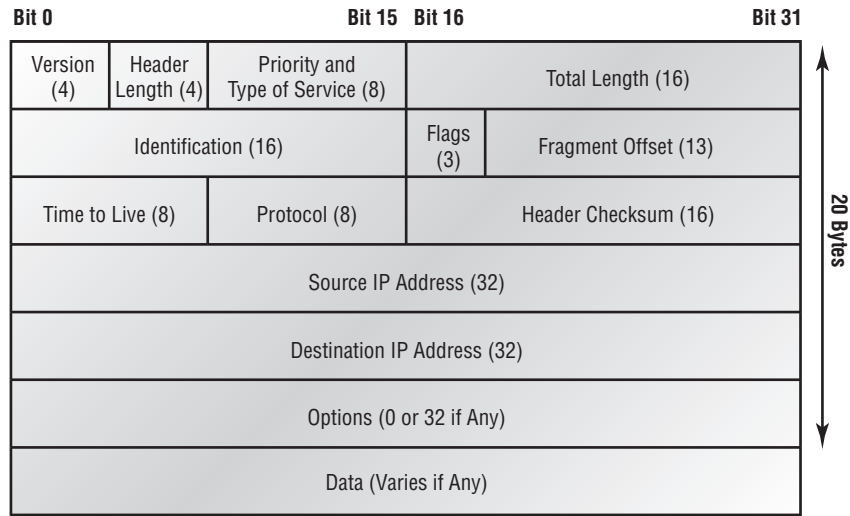
FIGURE 6.7 IP header
