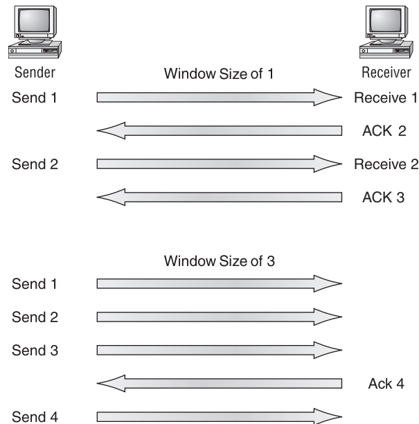
FIGURE 2.6 Windowing
