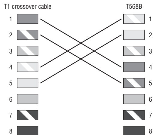
FIGURE 3.24 A T1 crossover cable
