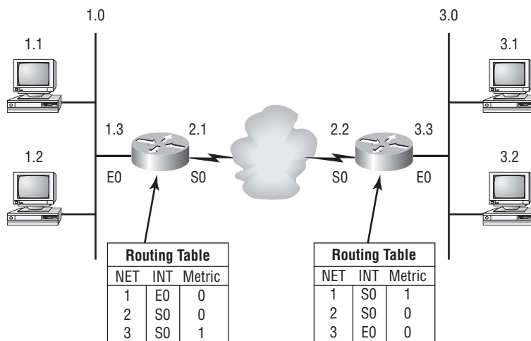
FIGURE 2.9 A router in an internetwork
