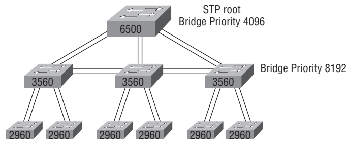
FIGURE 11.11 An optimal hierarchical switch design
