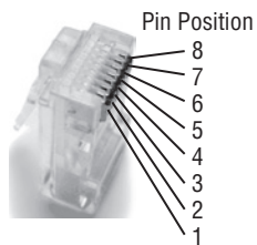
FIGURE 3.5 The pin-outs in an RJ-45 connector
