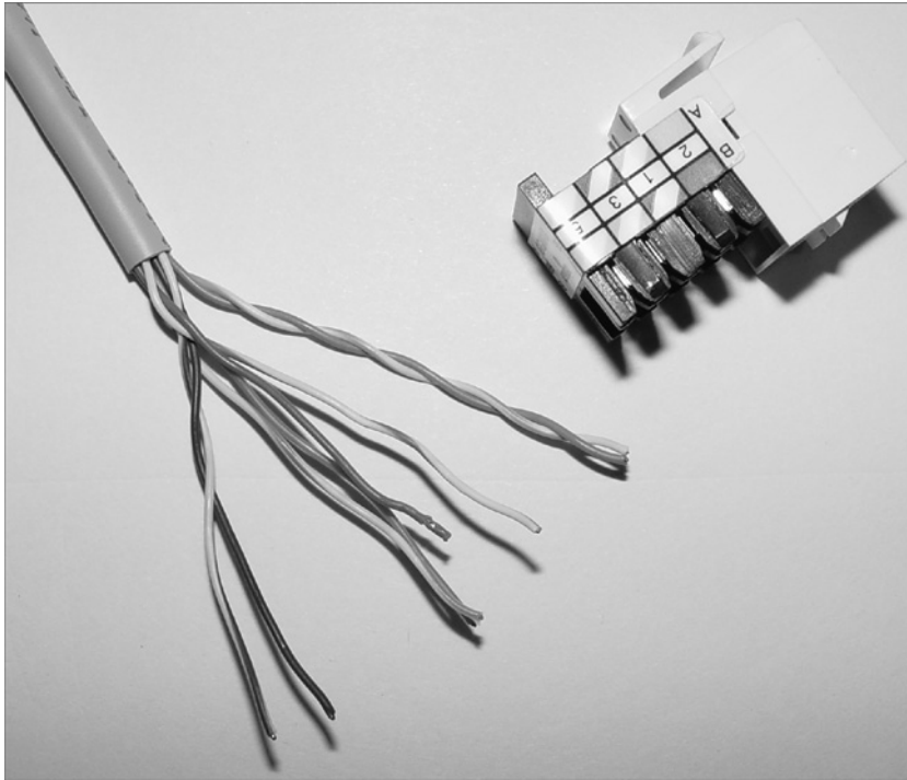
FIGURE 3.3 Cat 5e UTP cable
