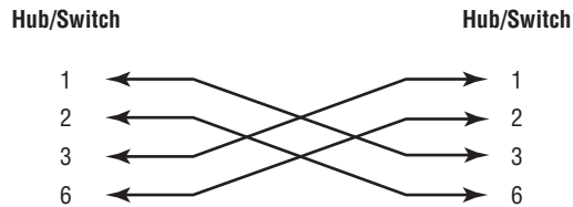
FIGURE 3.22 Crossover Ethernet cable
