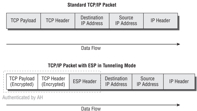
FIGURE 13.6 TCP/IP packet in IPSec tunnel mode with ESP
