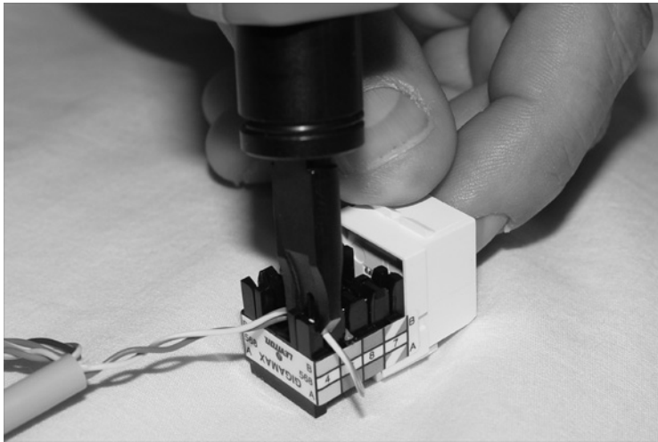
FIGURE 18.14 Using a punch-down tool on a small 110 block
