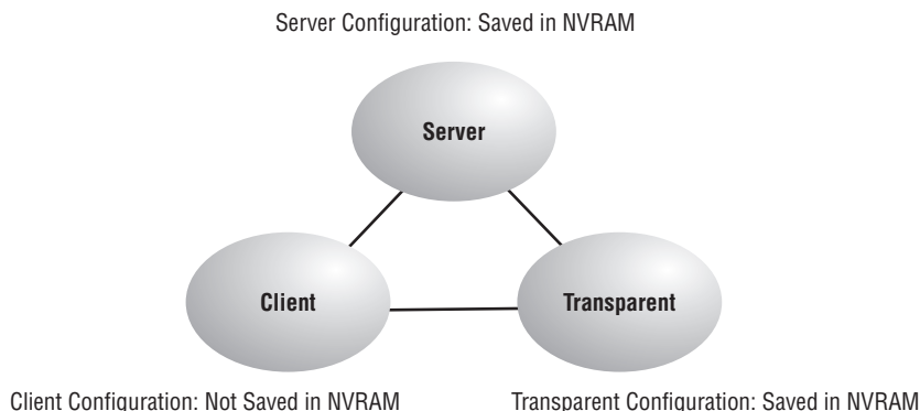
FIGURE 11.17 VTP modes
