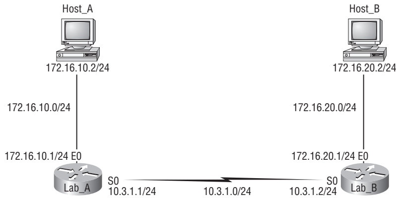
FIGURE 10.6 A discontinuous network
