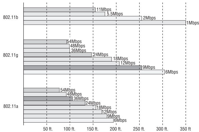
FIGURE 12.7 Range comparisons of 802.11 standards
